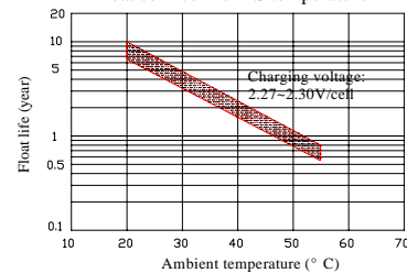
Float service life V'S temperature
