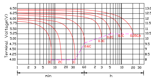
DISCHARGE CHARACTERISTICS AT 25° C(77° F)
